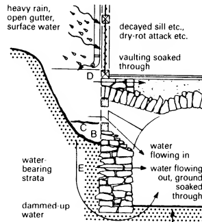
⑦ Main points of attack by pressurised water
